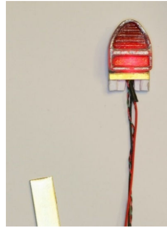
A slot in the mounting block takes the 6mm wide stalk.
